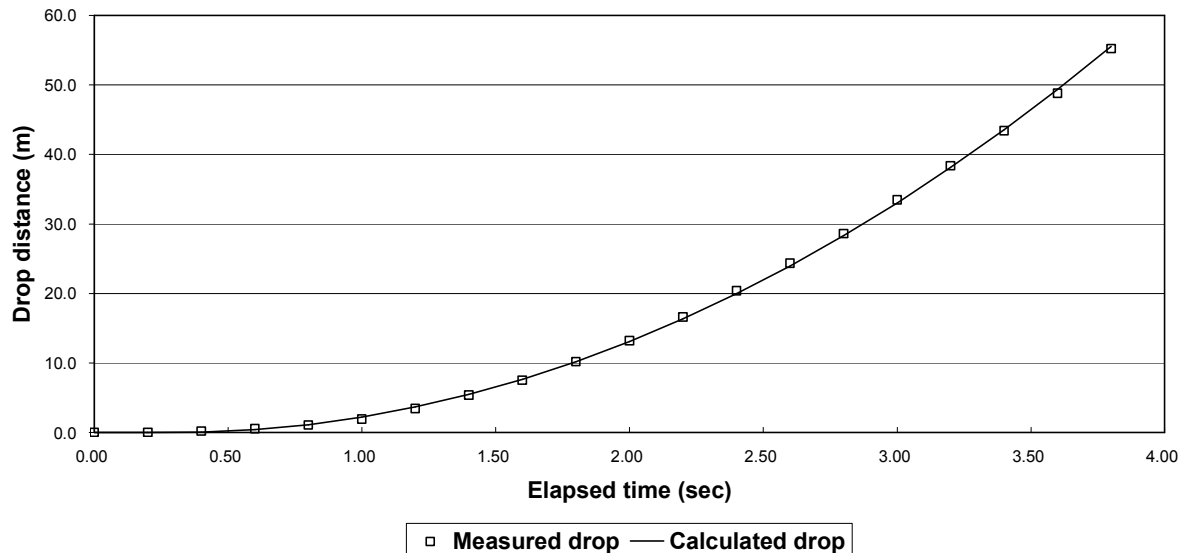
WTC 7 COLLAPSE Assumed constant acceleration: 9.1 m/s 2 Assumed start time: 0.3 seconds
